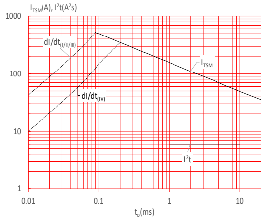
FIG.6: Non-repetitive surge peak on-state current for a sinusoidal pulse with width t_p < 20\text{ms} , and corresponding value of I^2t ( I - II - III: di/dt < 50\text{A}/\mu\text{s} ; IV: di/dt < 40\text{A}/\mu\text{s} )
