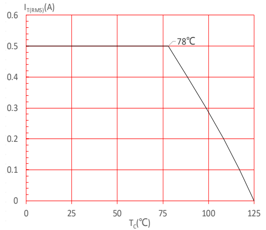
FIG.4: On-state characteristics
