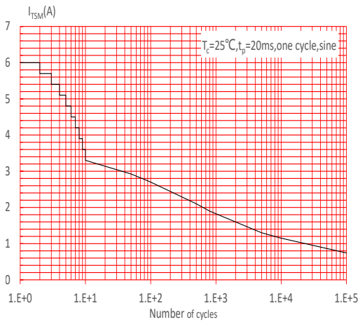
FIG.5: Non-repetitive surge peak on-state current for a sinusoidal pulse with width t_p < 20\text{ms} , and corresponding value of I^2t ( I - II : di/dt < 50\text{A}/\mu\text{s} ; III-IV : di/dt < 20\text{A}/\mu\text{s} )
