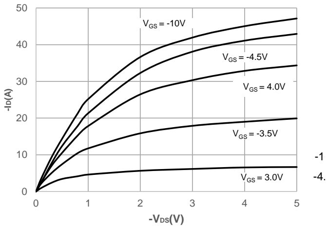
Figure 1: Output Characteristics
