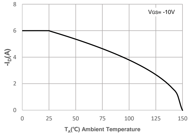
Figure 10: Maximum Continuous Driand Current vs. Ambient Temperature
