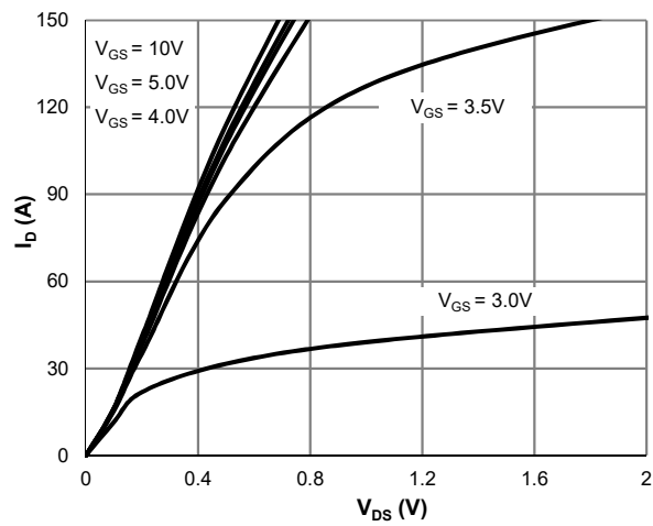
Figure 1: Saturation Characteristics
