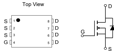
Pin Configuration
